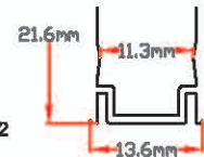
LNF-Clips-1-12 Mounting clip/Al., direct type, for LNT -PVC-SF1220/TF1212
