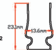
LNF-Clips-4-12 Mounting clip/Steel, plus type, for LNT -PVC-SF1220/TF1212
