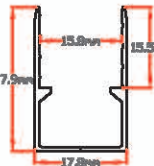
LNF-Clips-3-16 Mounting clip/Al., plus type, for LNT -PVC-TF1616
