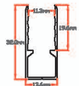
LNF-Clips-3-12 Mounting clip/Al., plus type, for LNT -PVC-SF1220/TF1212
