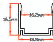
LNF-Clips-1-16 Mounting clip/Al., direct type, for LNT -PVC-TF1616
