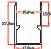
LNF-Clips-3-16 Mounting clip/Al., plus type, for LNT -PVC-TF1616
